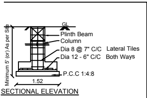
SECTIONAL ELEVATION
