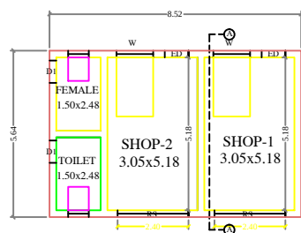
GROUND FLOOR
