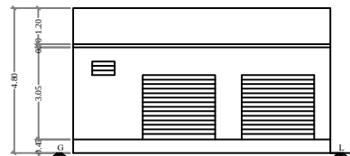
ELEVATION FACING WEST
