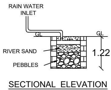
SECTIONAL ELEVATION
