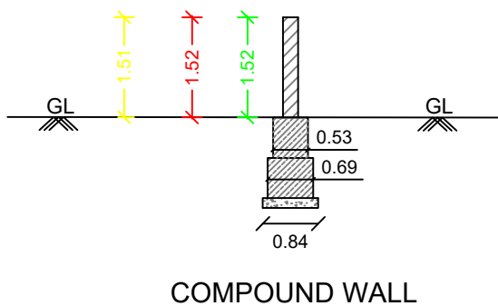
COMPOUND WALL
