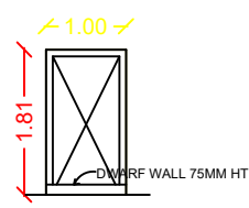
WICKET GATE
