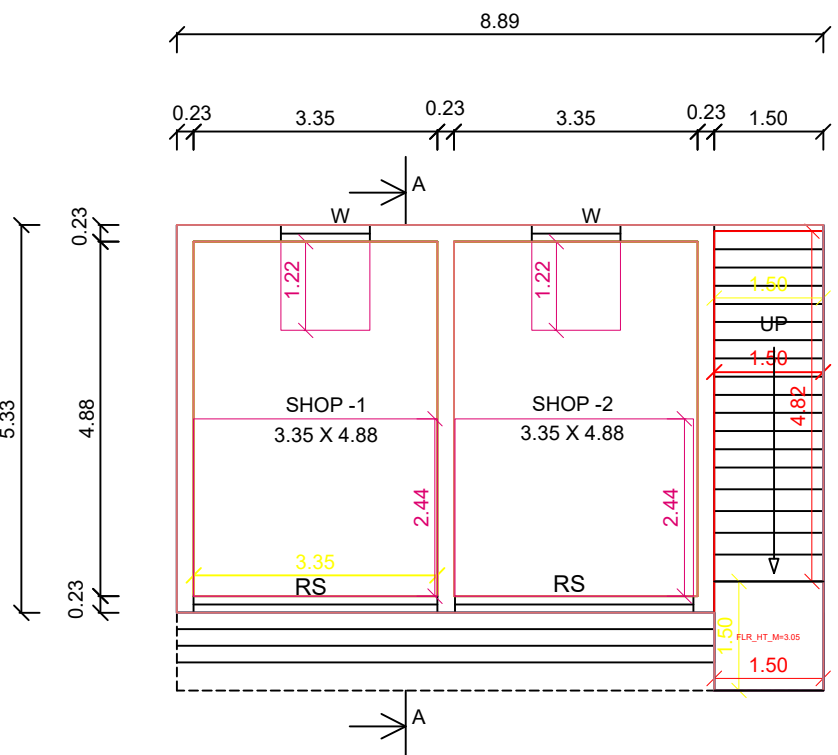
GROUND FLOOR SHOP PLAN
