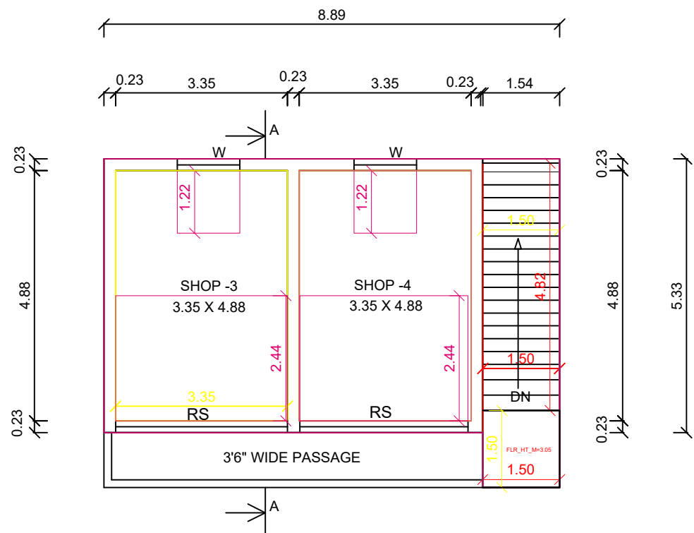
FIRST FLOOR SHOP PLAN
