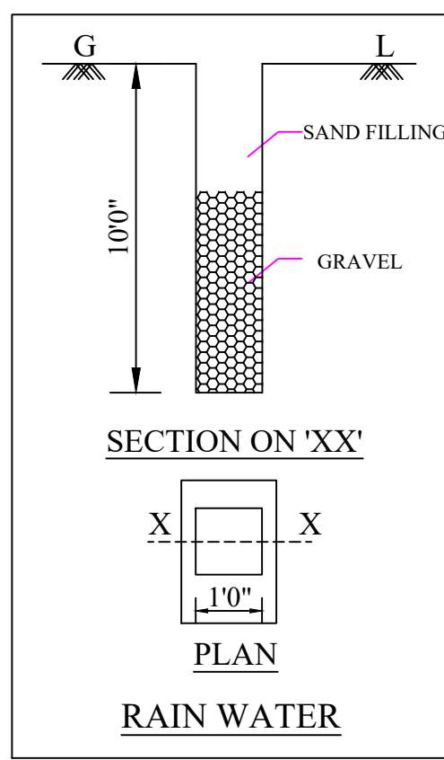
RAINWATER HARVESTING
