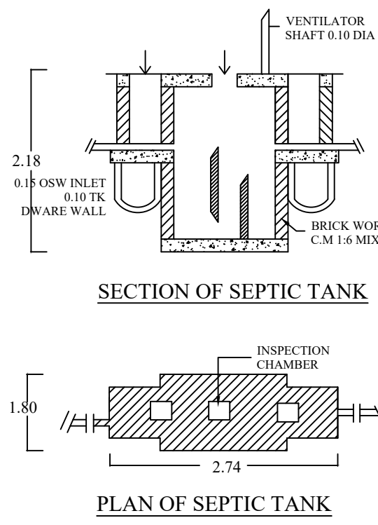
SEPTIC TANK
