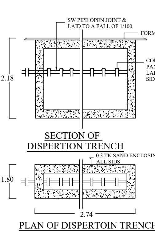
DISPERSION TRENCH
