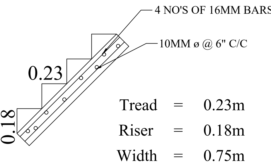
STAIRCASE DETAILS
