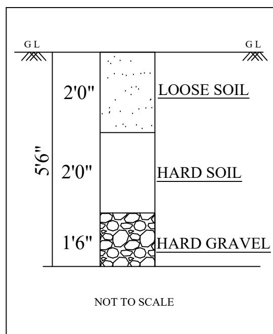
TRIAL PIT
