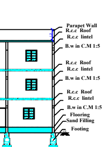
SECTION ON "AA"
