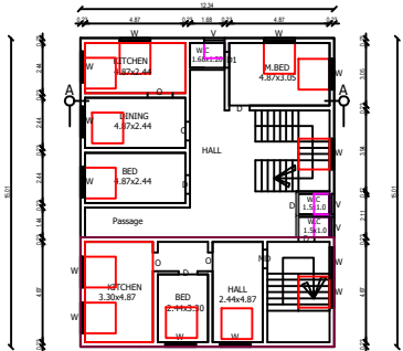
PRO SECOND FLOOR PLAN
