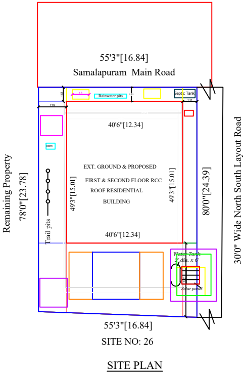
SITE PLAN
