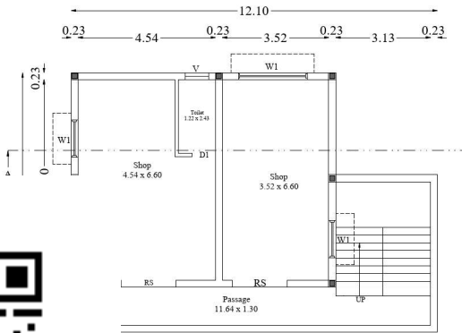
First Floor Plan Floor-01
