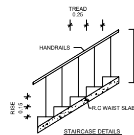
STAIRCASE DETAILS
