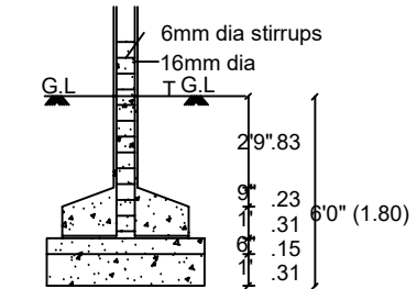
COLUMN FOUNDATION DETAIL
