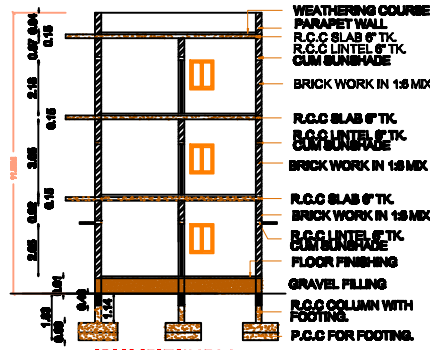
CROSS SECTION AT A-A
