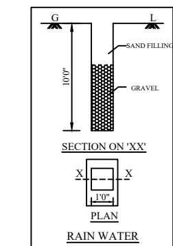
RAINWATER HARVESTING
