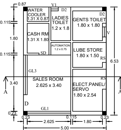
PROPOSED GF OFFICE BUILDING PLAN
