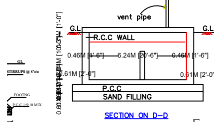
SUMP DETAIL
