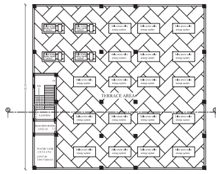
TERRACE FLOOR
