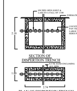
DISPERSION TRENCH
