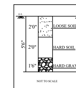
TRIAL PIT
