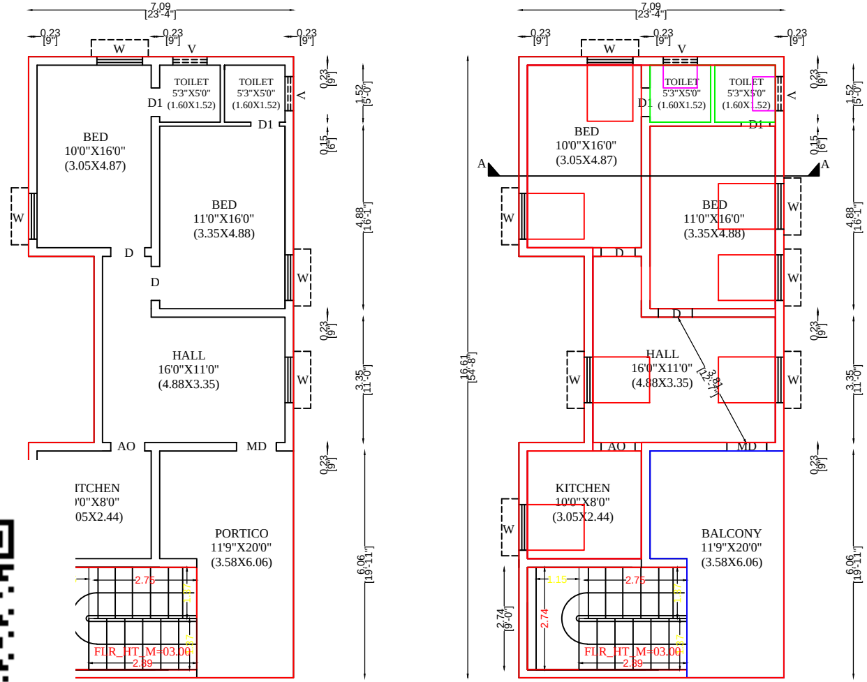
GROUND FLOOR
