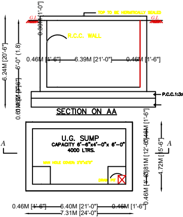
SUMP DETAIL SCALE 1"=4'0"
