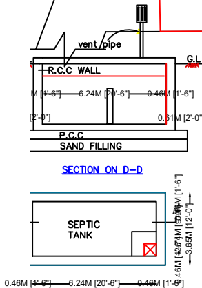
PLAN OF SEPTIC TANK SCALE 1"=2'0"
