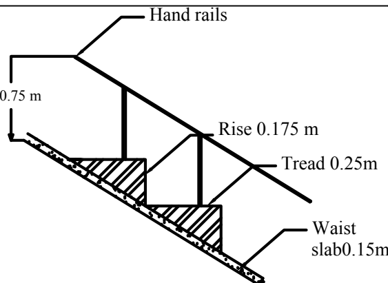
STAIRCASE DETAILS
