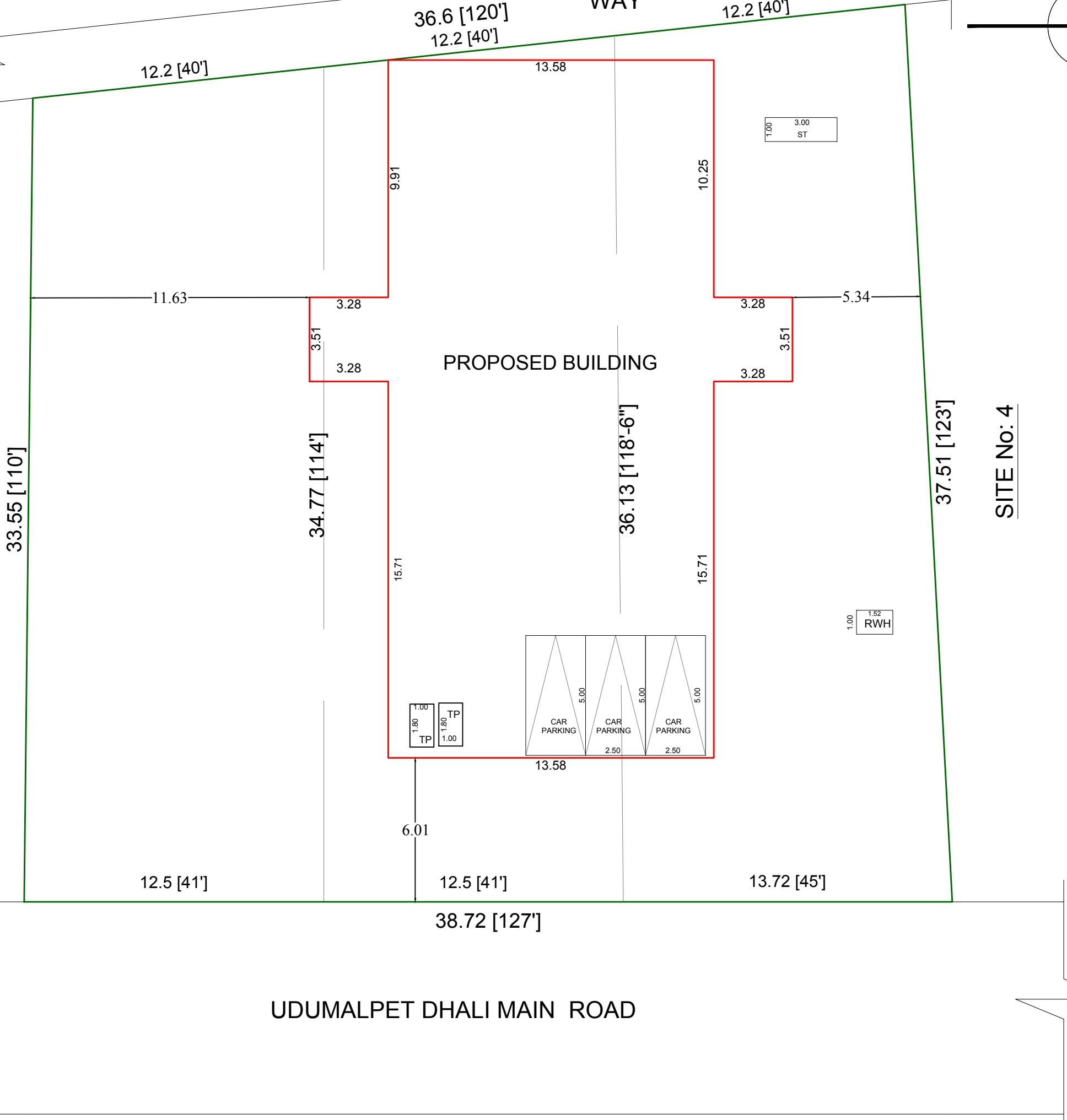
SITE PLAN
