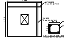
SECTION DETAILS OF SEPTIC TANK
