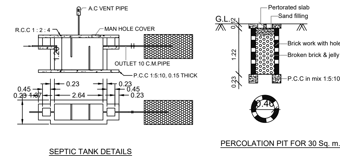
SEPTIC TANK DETAILS
