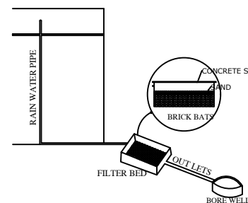
RAIN WATER HAVESTING TANK
