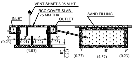
SECTION ON SEPTIC TANK & DISP-TRENCH
