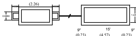
PLAN ON SEPTIC TANK & DISP-TRENCH
