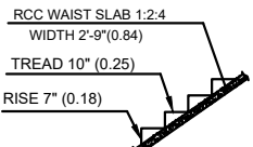
SCALE 1:50
