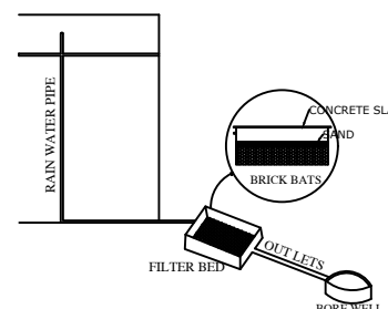
RAIN WATER HARVESTING TANK
