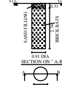
DETAILED PLAN OF RAINWATER PERCOLATION & COLLECTION PIT
