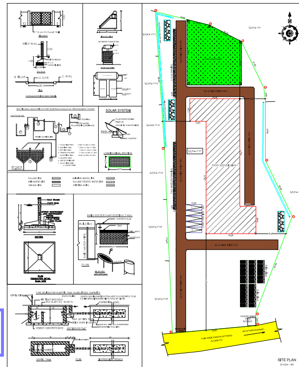
SITE PLAN
