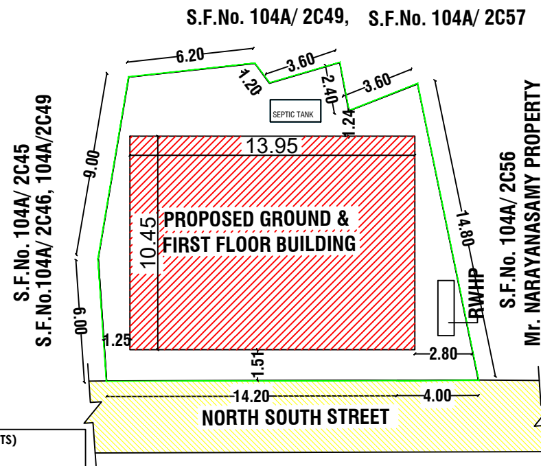
SITE PLAN
