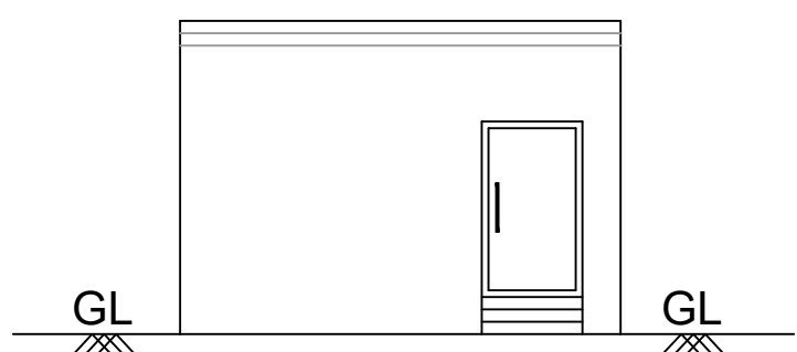
SOUTH SIDE ELEVATION BLOCK 2 (SCALE = 1:100)
