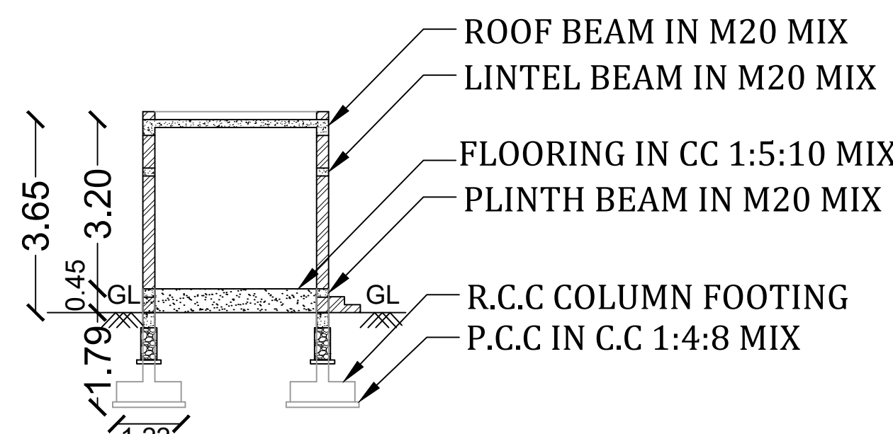
SECTION C-C BLOCK 3 (SCALE = 1:100)
