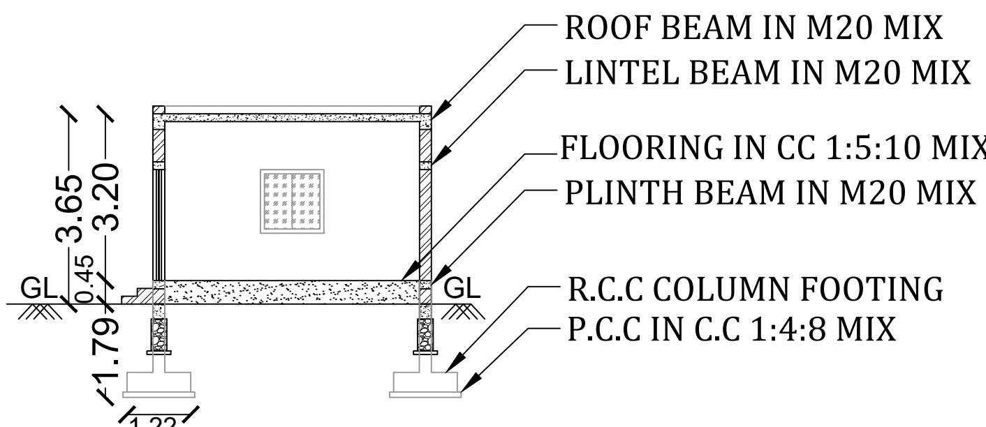
SECTION B-B BLOCK 2 (SCALE = 1:100)
