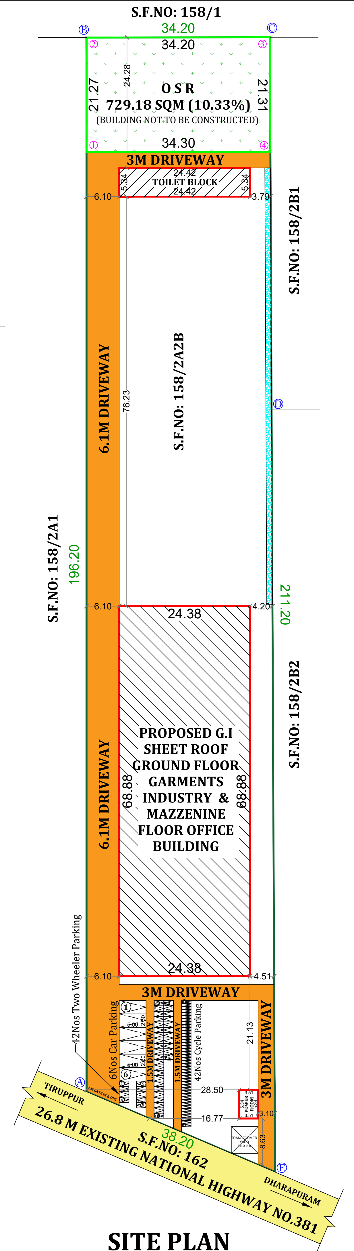
SITE PLAN (SCALE = 1:400)
