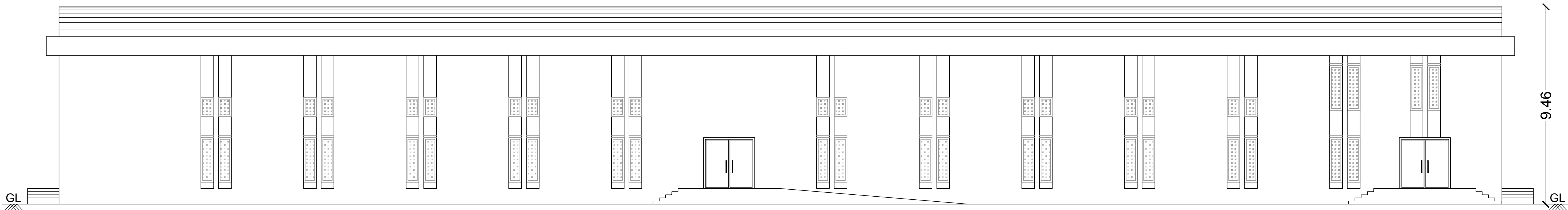
WEST SIDE ELEVATION BLOCK 1 (SCALE = 1:100)
