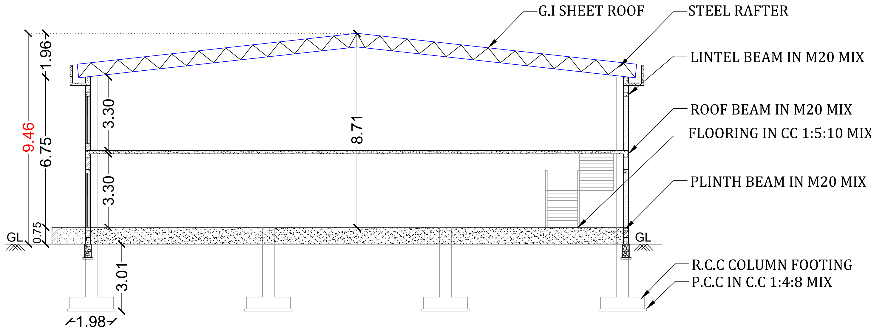
SECTION A-A BLOCK 1 (SCALE = 1:100)
