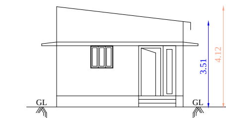
FRONT ELEVATION
