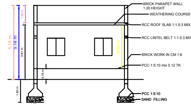
SECTION " AB "
