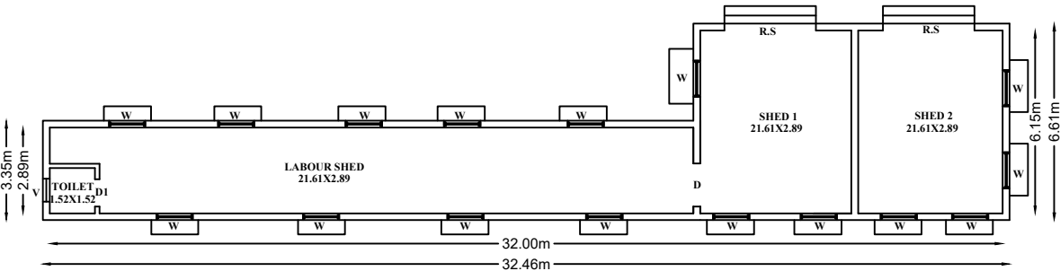
PROPOSED BUILDING PLAN
