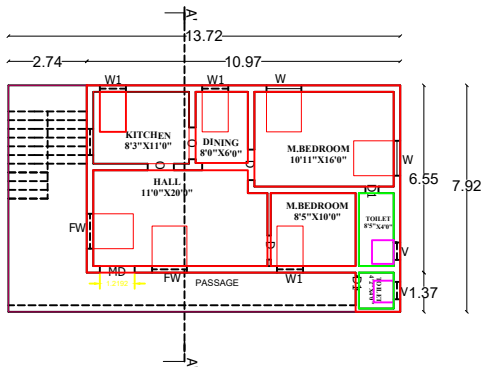
FIRST FLOOR PLAN FACING NORTH
