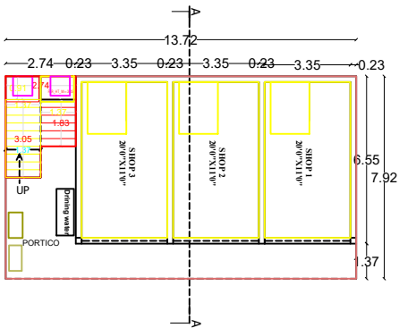
GROUND FLOOR PLAN FACING NORTH
