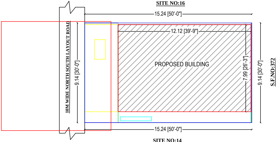
SITE PLAN
