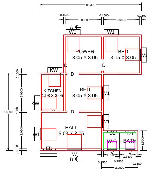
GROUND PLAN (SCALE 1:100)
