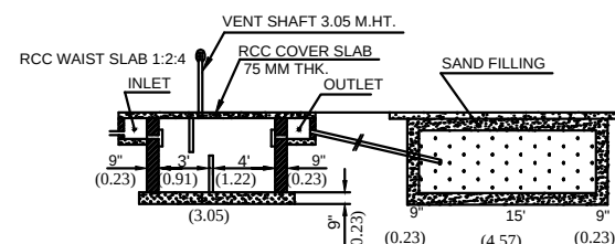
SECTION ON SEPTIC TANK & DISP-TRENCH
