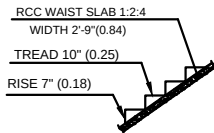
STAIRCASE DETAIL SCALE 1:50
