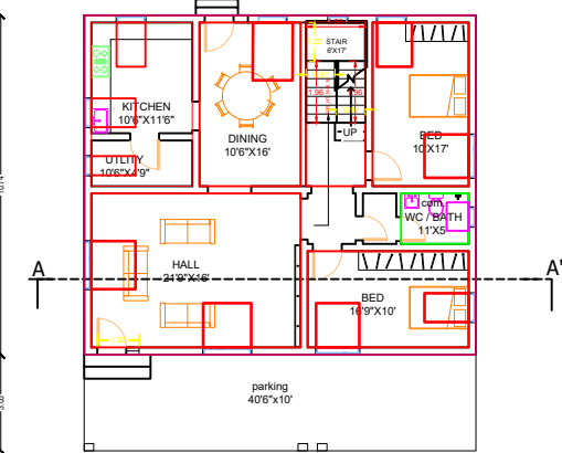
GROUND FLOOR PLAN FACING NORTH
