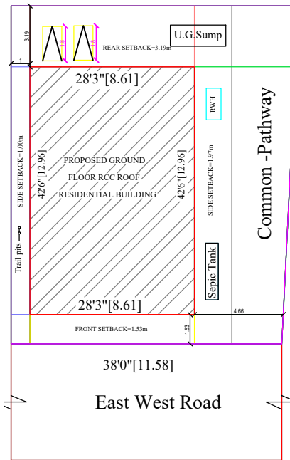
SITE PLAN
