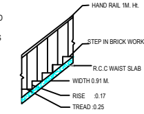
STAIR DETAIL
