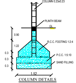
COLUMN DETAILS
