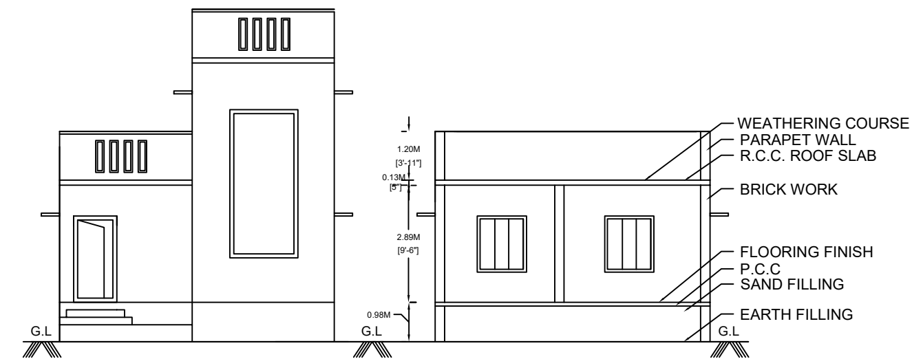
FRONT ELEVATION
