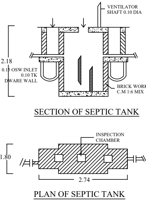
SEPTIC TANK
