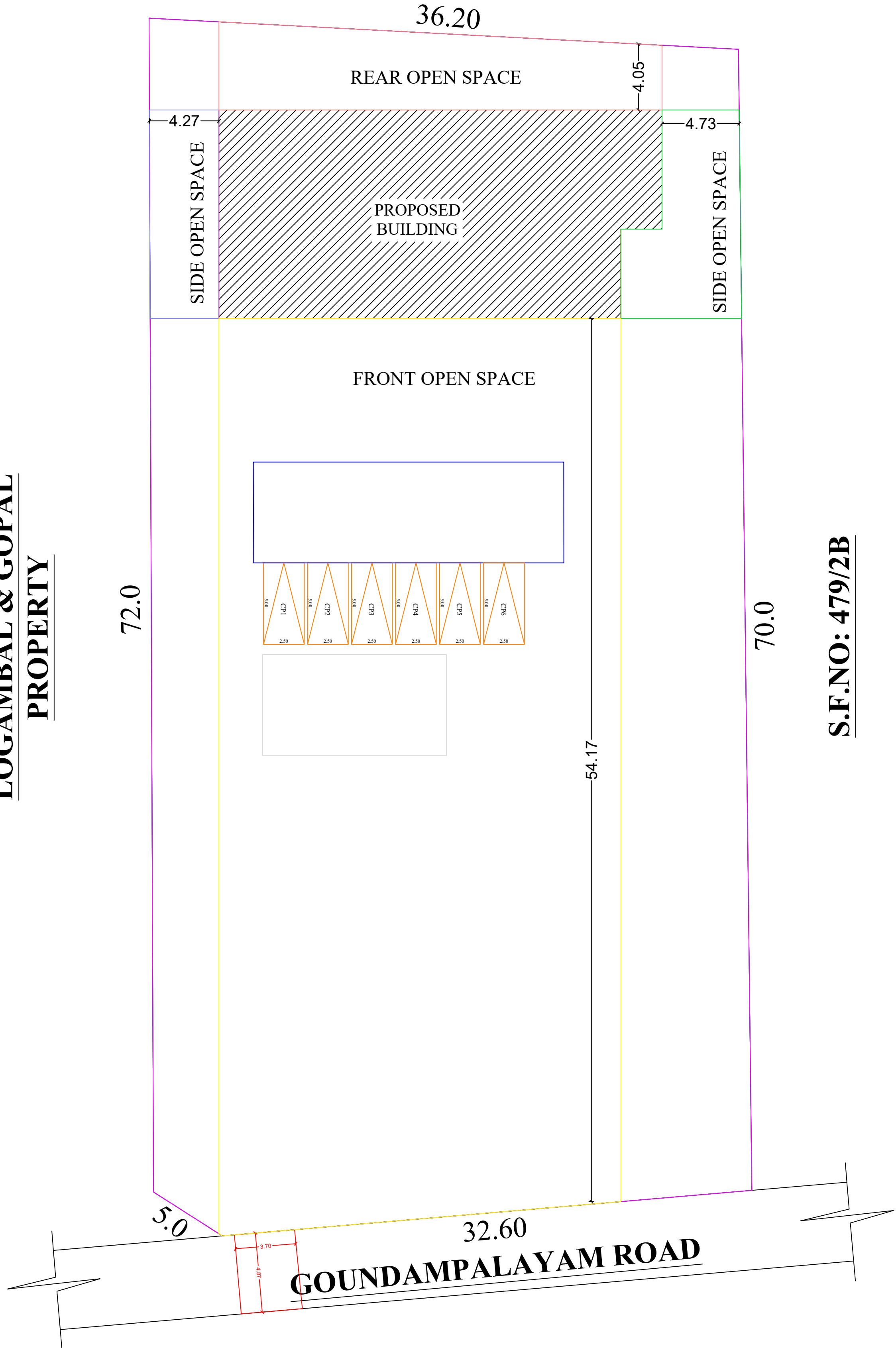
SITE PLAN
