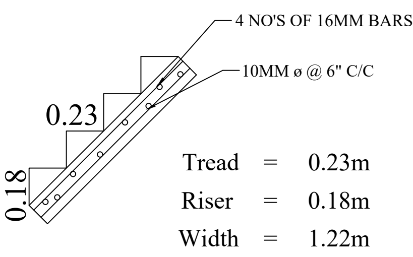
STAIRCASE DETAILS
