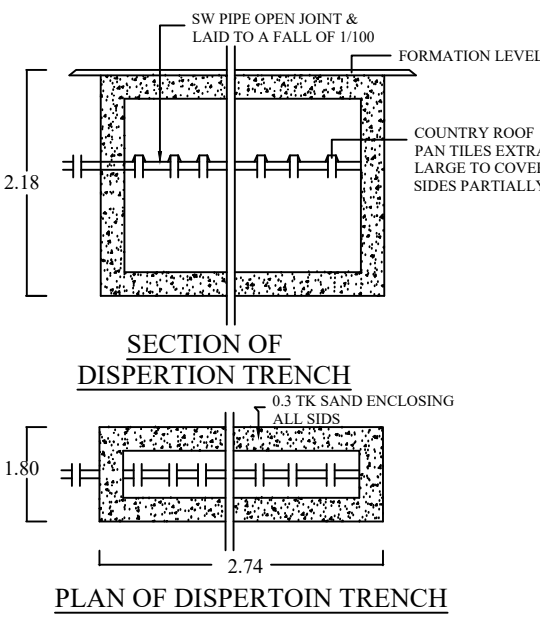
DISPERSION TRENCH
