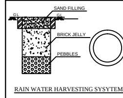
RAIN WATER HARVESTING SYSYTEM
