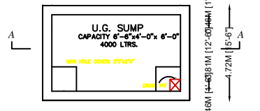
SUMP DETAIL SCALE 1"=4'-0"
