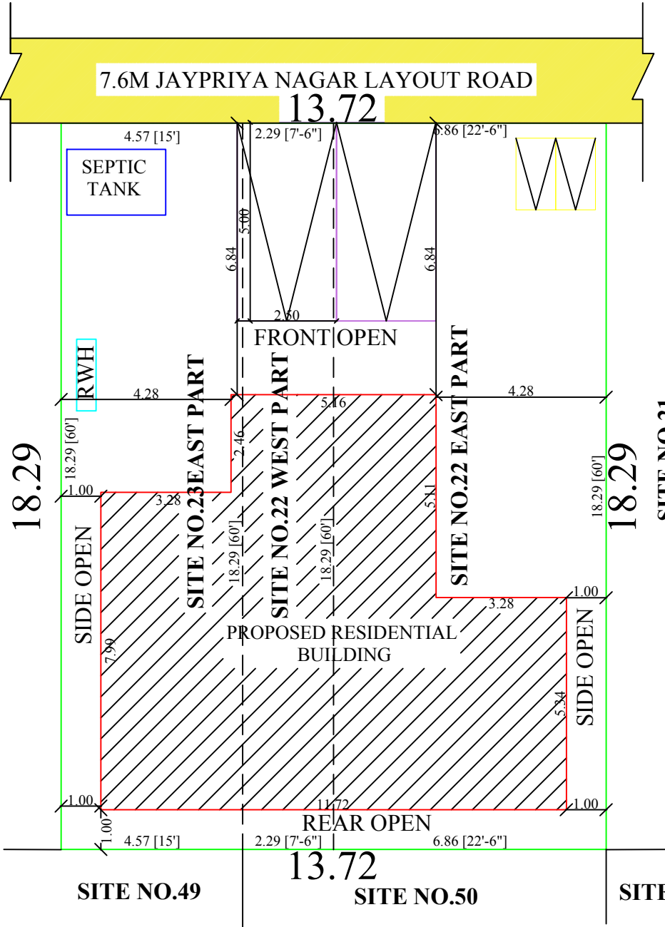
SITE PLAN(1:100)
