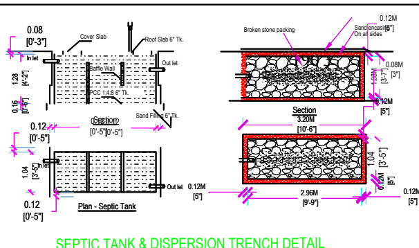
SEPTIC TANK & DISPERSION TRENCH DETAIL
