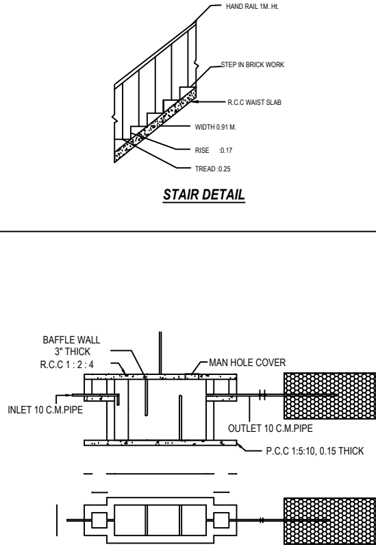
SEPTIC TANK & TRENCH
