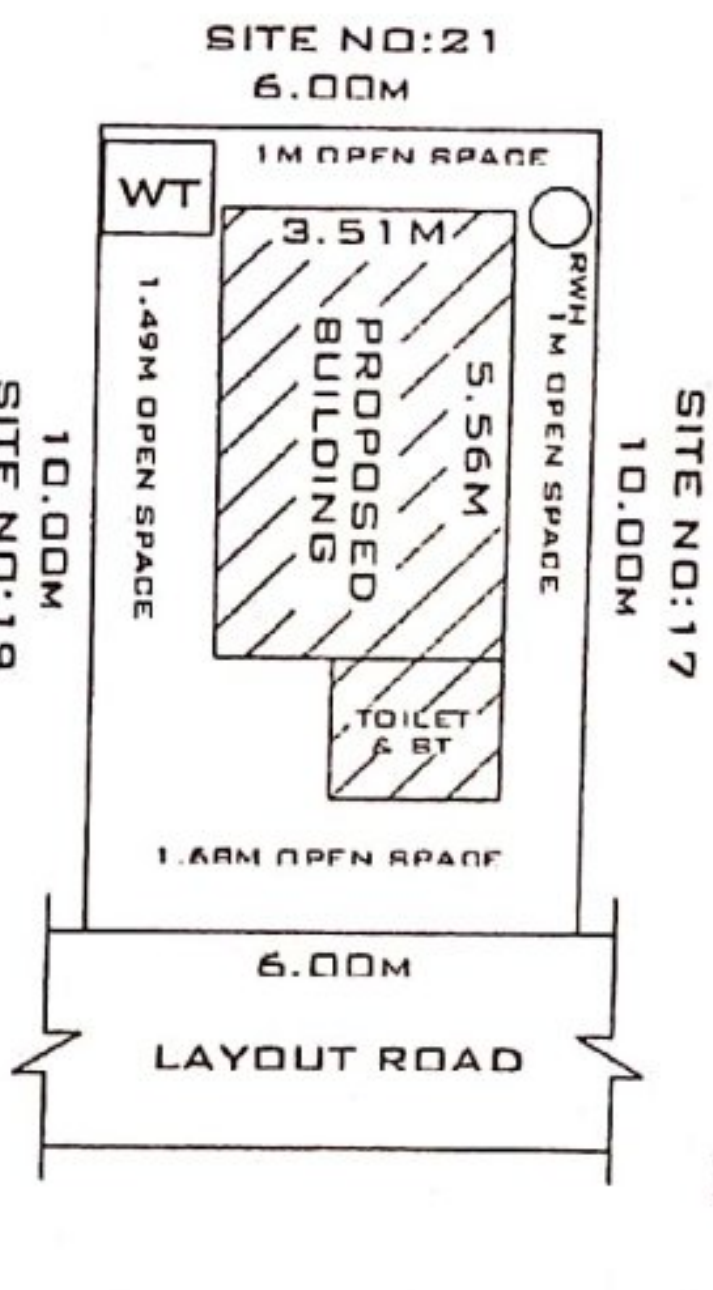
SITE PLAN
