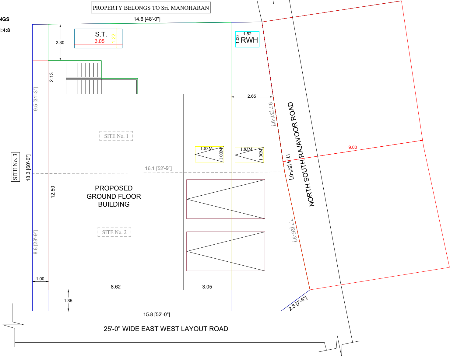
SITE PLAN
