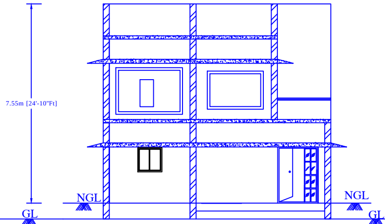
FRONT EAST ELEVATION
