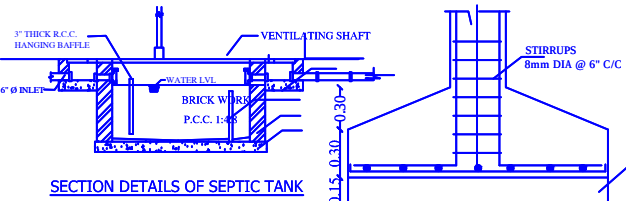
SECTION DETAILS OF SEPTIC TANK
