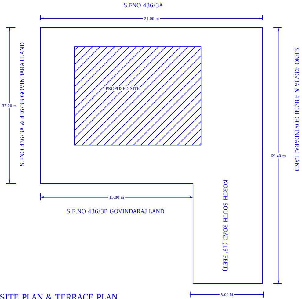
SITE PLAN & TERRACE PLAN
