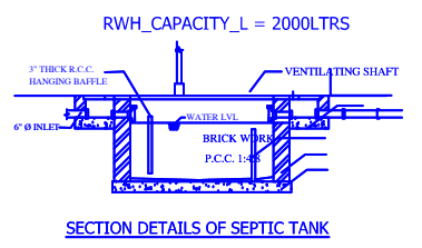
SECTION DETAILS OF SEPTIC TANK
