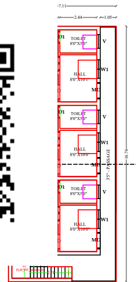
FLOOR-FIRST
