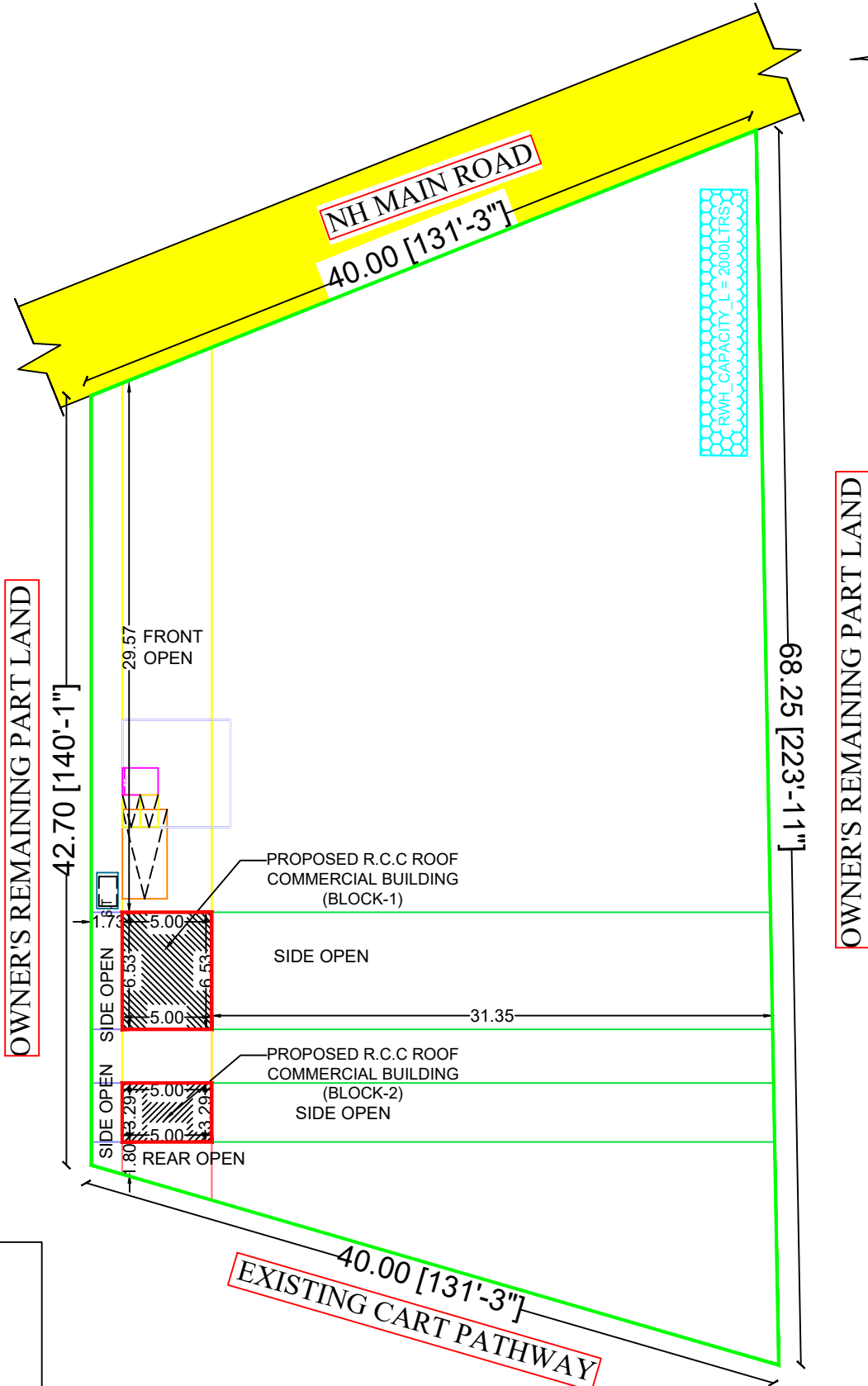
SITE PLAN
