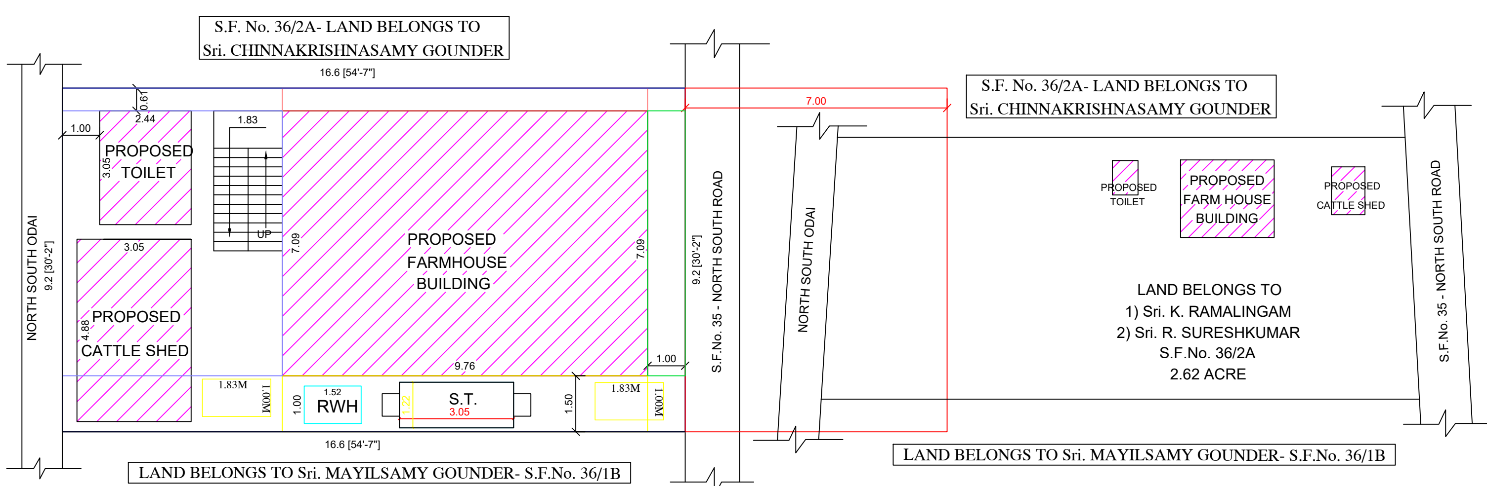
SITE PLAN - MEANT FOR FARM HOUSE
