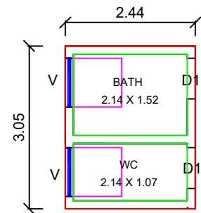
TOILET BLOCK PLAN
