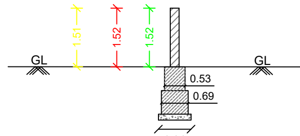
COMPOUND WALL
