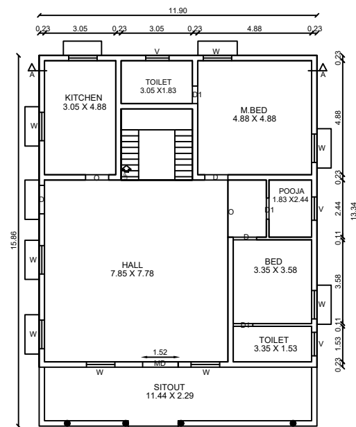
GROUND FLOOR BUILDING PLAN
