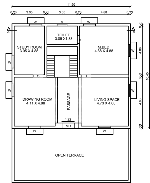
FIRST FLOOR BUILDING PLAN
