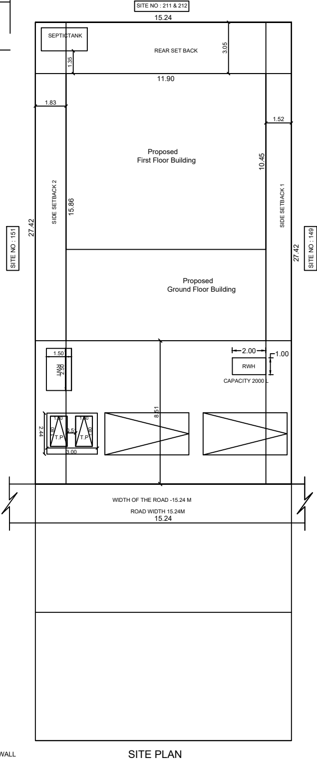
SITE PLAN
