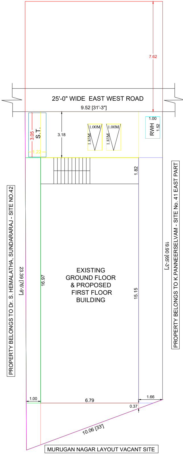
SITE PLAN
