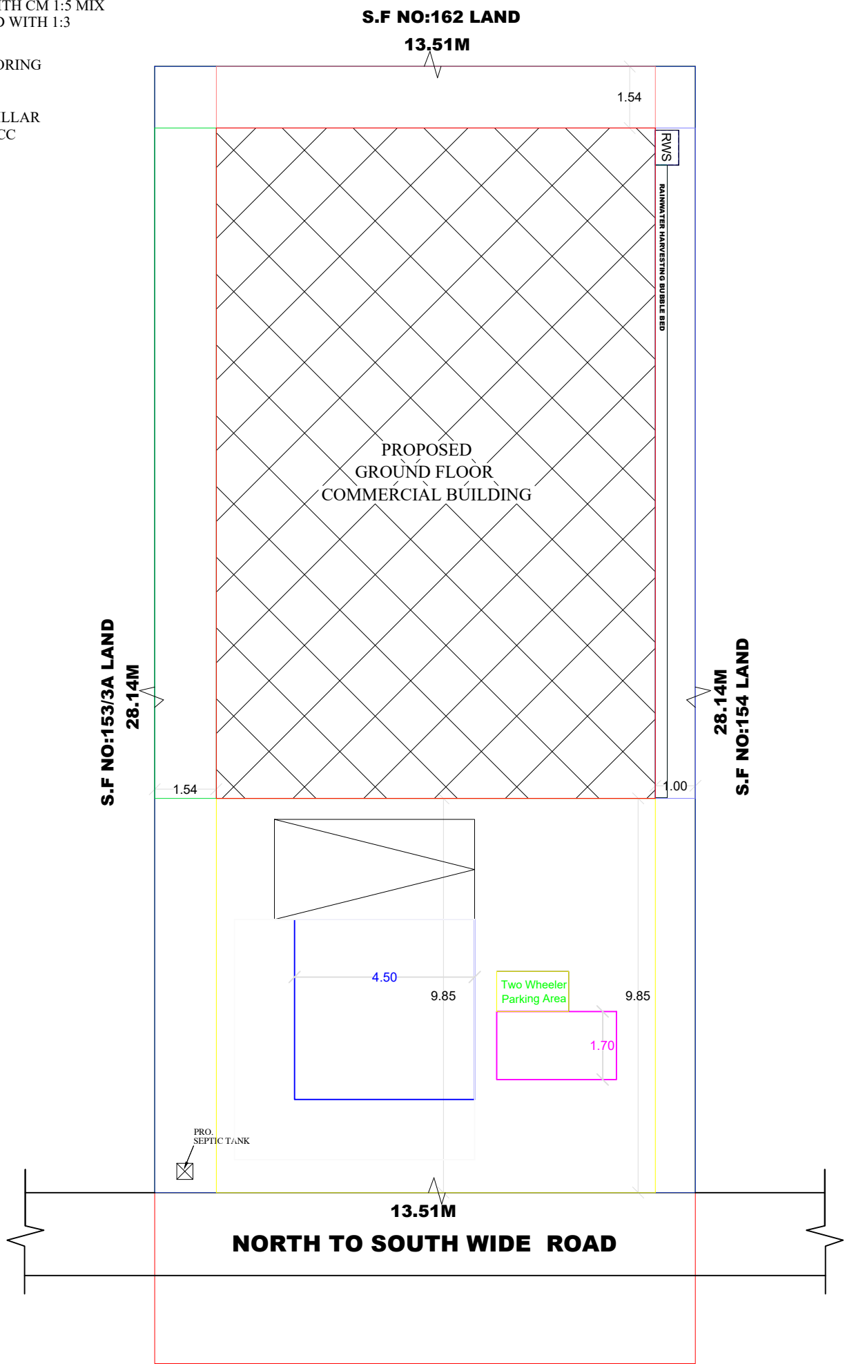
SITE PLAN (SCALE 1:1)
