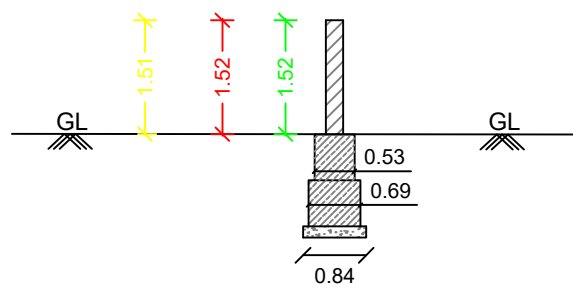
COMPOUND WALL
