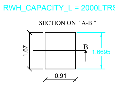
DETAILED PLAN OF RAINWATER PERCOLATION AND COLLECTION PIT
