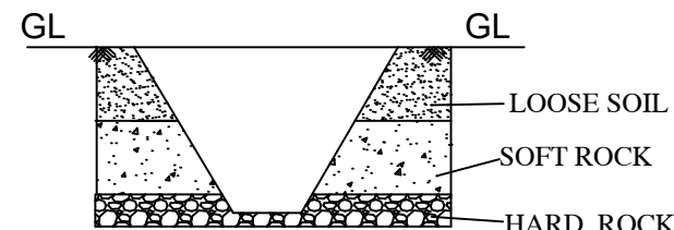
TRIAL PIT
