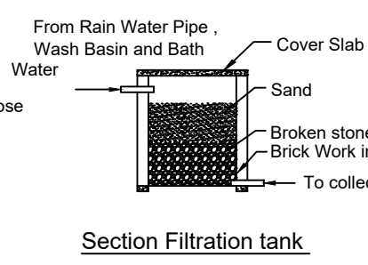
Section Filtration tank
